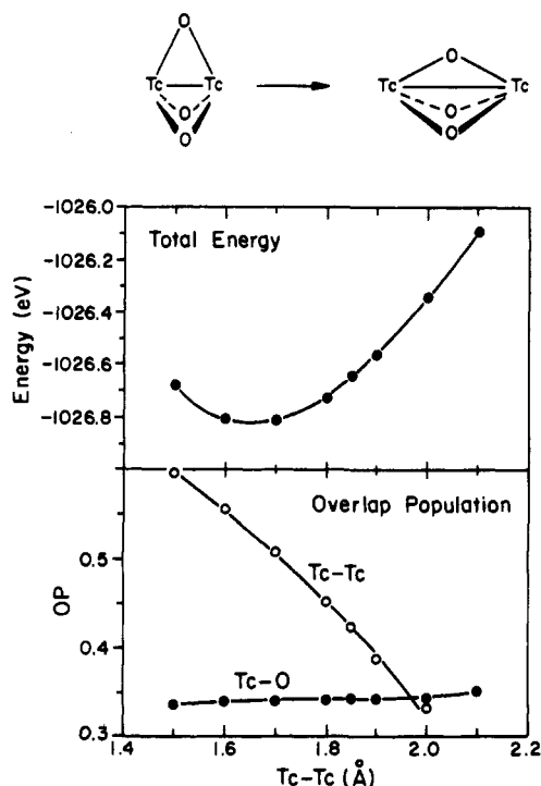
Figure 10. Energy and Tc-Tc and Tc-O OP vs Tc-Tc distance when Tc-O distance is kept as a constant.
